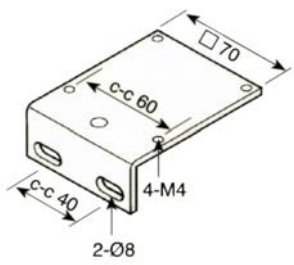
300-WM Wall Mount
